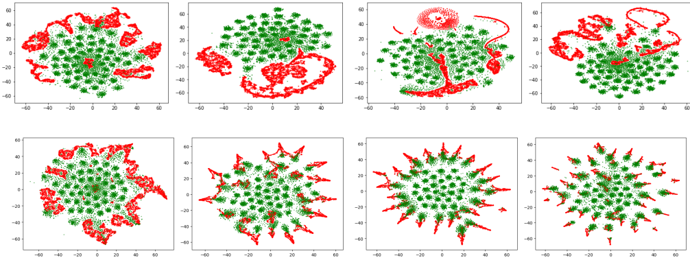
Figure 2: t-SNE plot of encoder output vectors (red) and samples from the Dirichlet prior (green) over epochs. First row corresponds to epochs 0,10,30,99 of GAN training; second row corresponds to those of MMD training.
